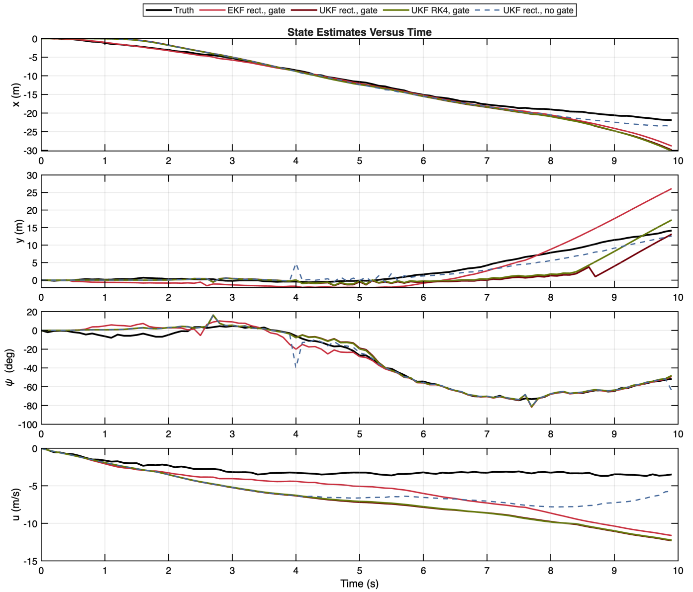
Fig. 4. State estimates versus time for the principal comparison cases. The gated filters maintain improved heading agreement, but their position and speed estimates drift as measurements are rejected.
