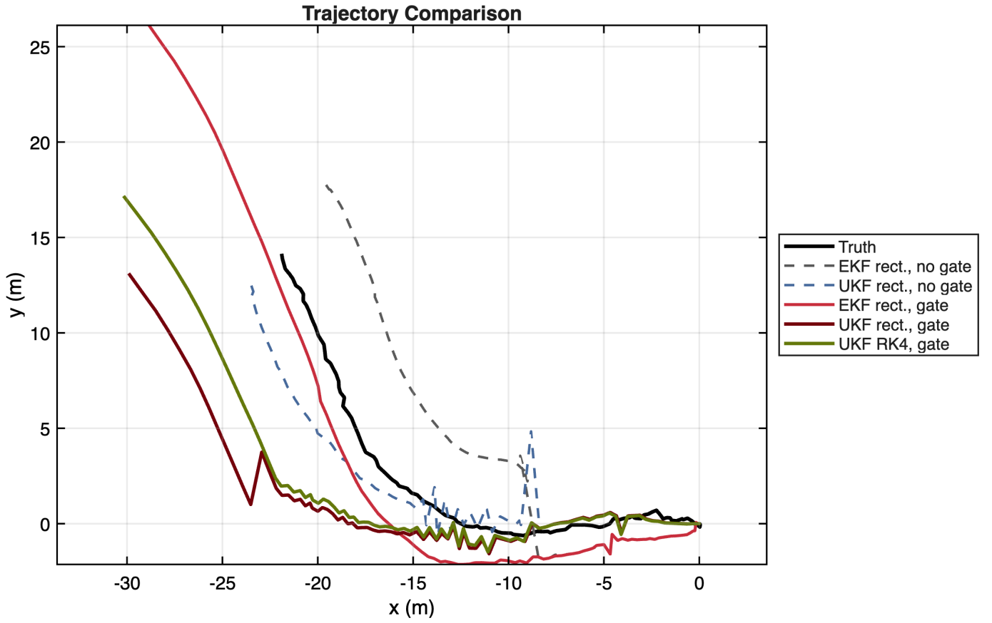
Fig. 2. Truth and estimated trajectories for the main filter configurations. The ungated UKF remains closest to the measured path, while the gated runs become increasingly prediction dominated late in the record.
