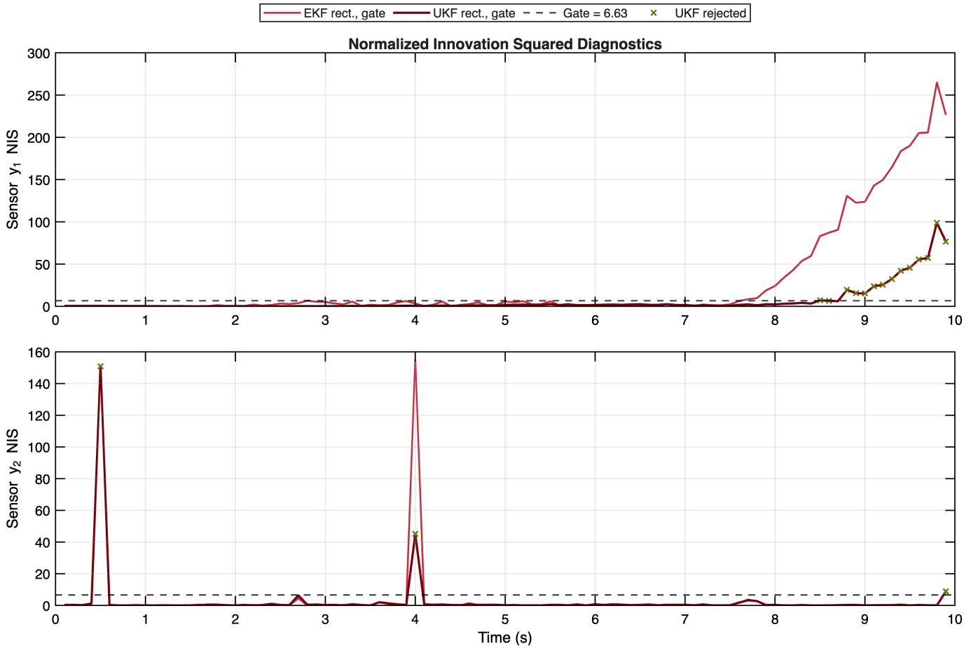
Fig. 3. Normalized innovation squared histories for both scalar sensors. The isolated y_2 spikes are clearly detectable, while the late growth in y_1 residuals explains the large number of range-measurement rejections.
