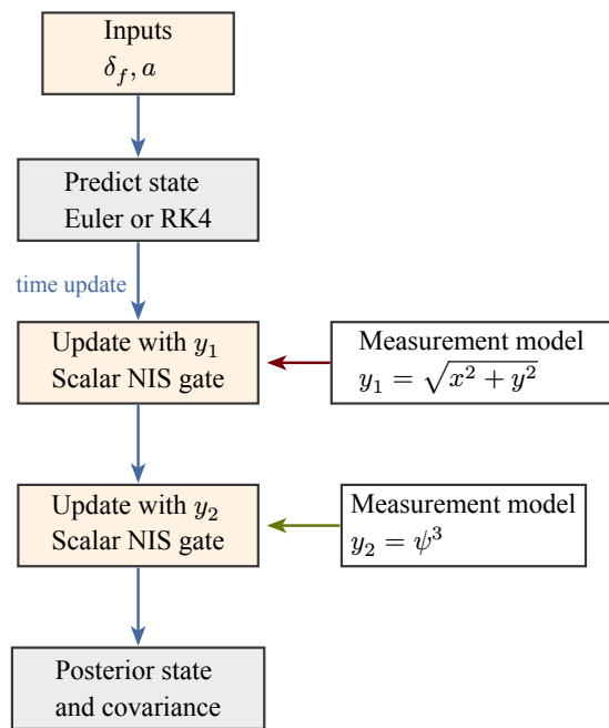
Fig. 1. Standalone CeTZ diagram of the sequential estimation workflow. The figure was authored separately, compiled to PDF, and then imported into the main IEEE-formatted document as a standard image asset.
