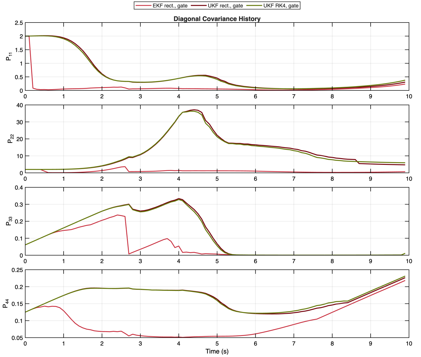
Fig. 5. Diagonal covariance histories for the gated EKF, gated rectangular UKF, and gated RK4 UKF. The UKF variants retain visibly larger uncertainty than the EKF, which is consistent with their stronger nonlinear treatment.
