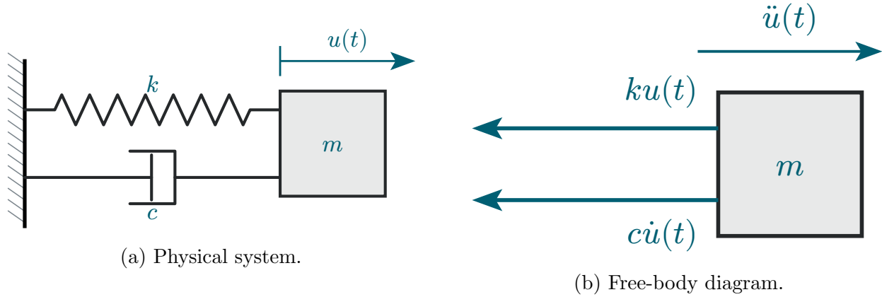
Figure 5: Mass-spring-damper vibrating system.
