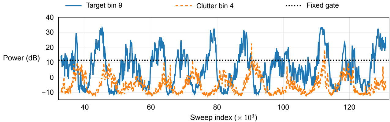
Figure D3. Measured target-bin and clutter-bin powers for every held-out window. The gate and receiver correction are frozen before sweep 32,768. File and tutorial pulse-frequency conventions conflict, so the horizontal axis retains sweep index. Powers are relative receiver quantities, not calibrated target cross sections.
