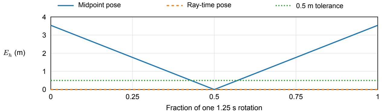
Figure D2. Calculated midpoint-pose error for constant translation at 11 kn over a 1.25 s rotation. The maximum is 3.537 m. Ideal ray-time mapping removes this prescribed translation error. The green line is the proposal's 0.50 m tolerance. These are model calculations, not Lund et al.'s measured residuals.
