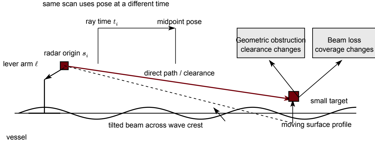
Figure B1. A moving radar and target change beam offset, direct-path clearance, and the pose used for mapping. Geometric obstruction, beam loss, and position distortion are distinct outcomes of the same state.
