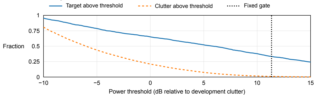
Figure D4. Measured fractions above candidate power thresholds in the held-out segment. The vertical line is the frozen development gate. Pooled clutter comprises ten non-target bins. Target-bin crossings are an observability proxy, without per-sweep target-visibility labels.
