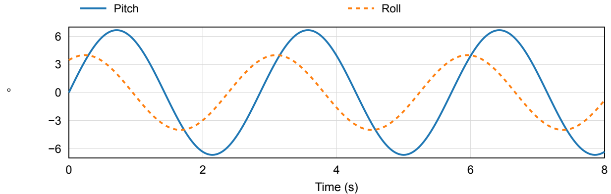
Figure C1. Computed roll and pitch for the stated forcing and response parameters. The modes determine the beam offset and radar-origin movement in Figure C2.
