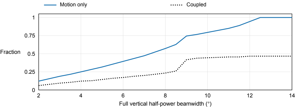
Figure C4. Computed phase fraction above the power gate as vertical beamwidth varies. The coupled curve retains wave-path attenuation, so recovering pointing coverage does not guarantee a usable return. Peak antenna gain is held fixed to isolate width; a hardware design must include its gain tradeoff.
