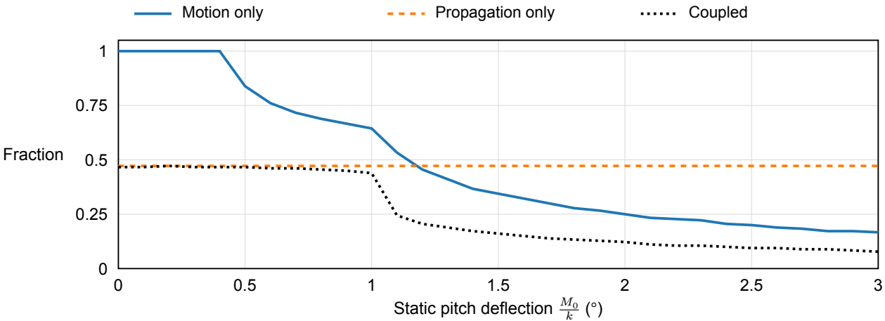
Figure C3. Computed phase fraction above the target-power gate as the static pitch deflection varies. The response gain remains 3.333, so the horizontal axis controls excitation amplitude rather than changing the natural frequency. The propagation-only curve uses a fixed radar platform.
