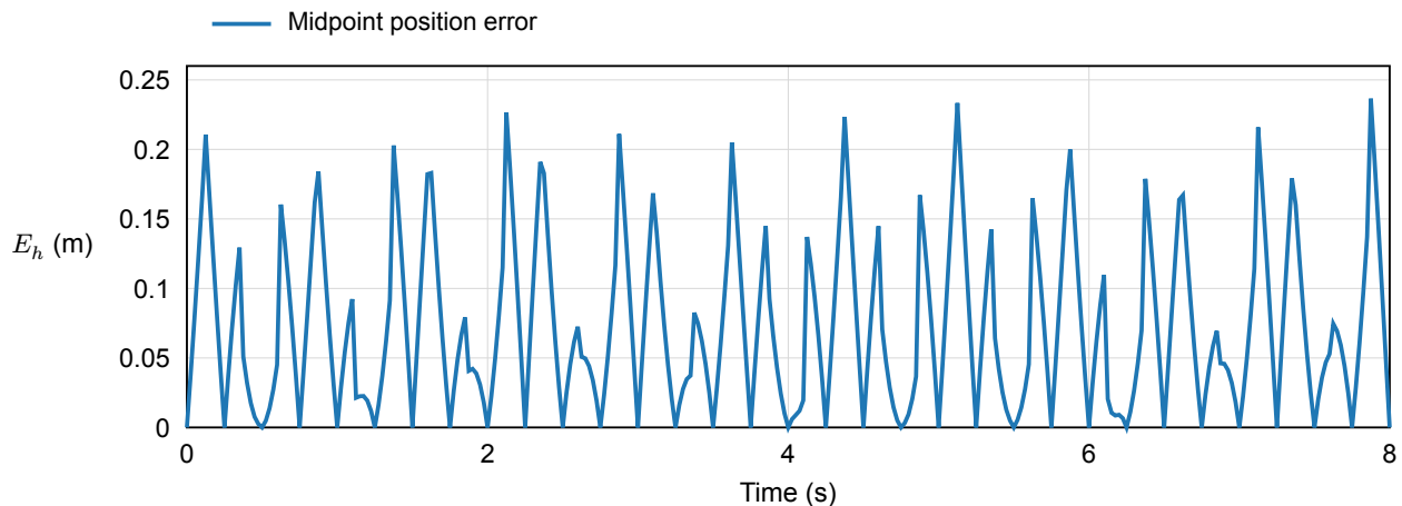
Figure C6. Computed midpoint reconstruction error over eight seconds using a known target-height plane. The error is evaluated at all time samples, including those rejected by the power gate, to isolate geometry. It is not conditional detected-return accuracy; the benchmark will report that quantity with the missed fraction.
