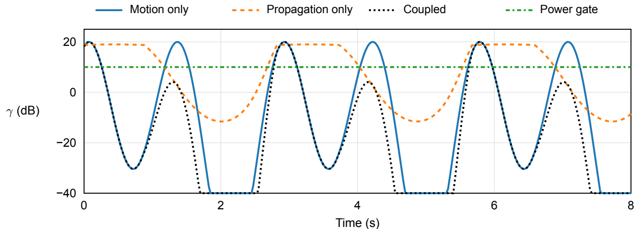
Figure C2. Target-power signal-to-noise ratio (SNR) proxy for motion-only, propagation-only, and coupled conditions. The green line is a prescribed power gate. Curves below -40 dB are clipped for display. This target-only power calculation does not report detector probability.
