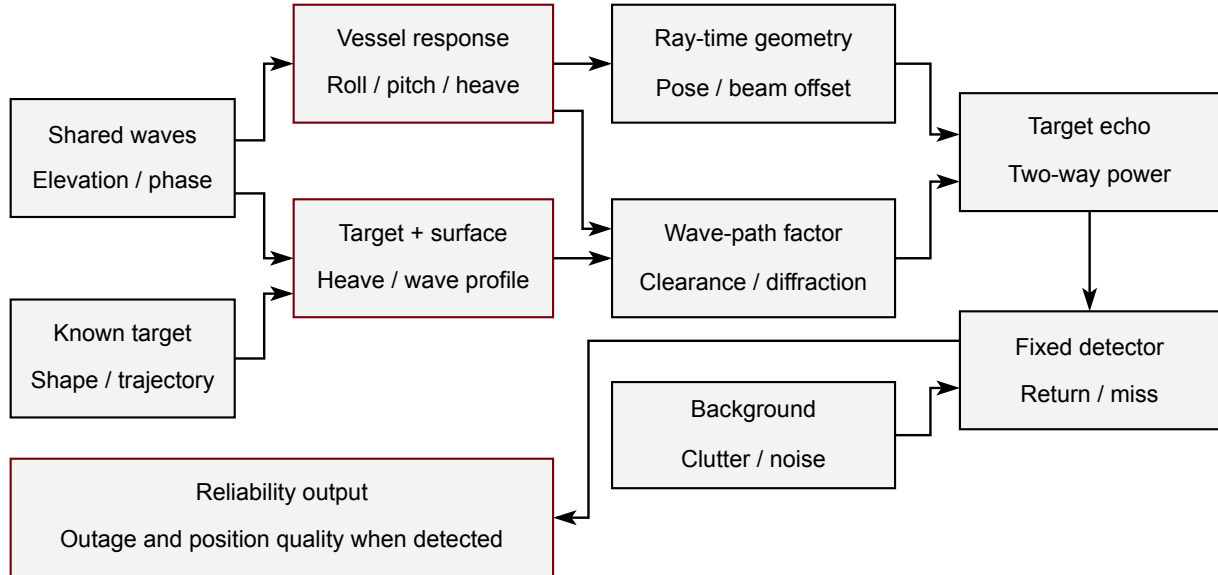
Figure A1. Shared forcing connects vessel motion and target state to acquisition-time geometry, propagation, and radar reliability. The same realization and clock must drive both branches. Radar cross section (RCS) specifies the target scattering term; position quality is assessed when the detector supplies a return.
