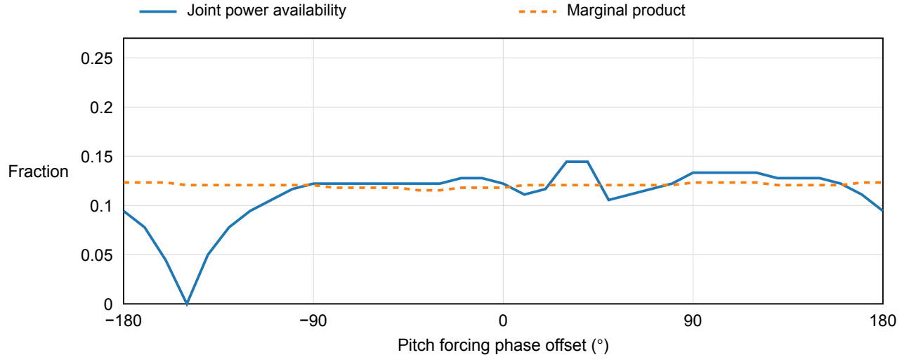
Figure C5. Computed joint power availability and the product of motion-only and propagation-only marginal fractions. The marginal product is an independence reference, not a joint radar model. Phase offsets give joint fractions from 0.000 to 0.144; the largest product discrepancy is 0.121. These differences motivate a common-state benchmark rather than establish field improvement.
