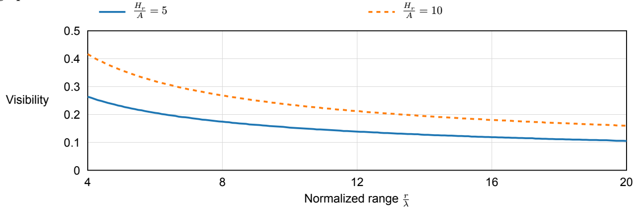
Figure D1. Calculated surface visibility using Wijaya and van Groesen's equations and Figure 3.4 parameter case. At \frac{r}{\lambda} = 10 , visibility is 0.153 for \frac{H_r}{A} = 5 and 0.235 for \frac{H_r}{A} = 10 . Doubling phase and radial resolution changes the curves by at most 0.0011. Surface visibility supplies a propagation baseline; it is not target detection probability.
