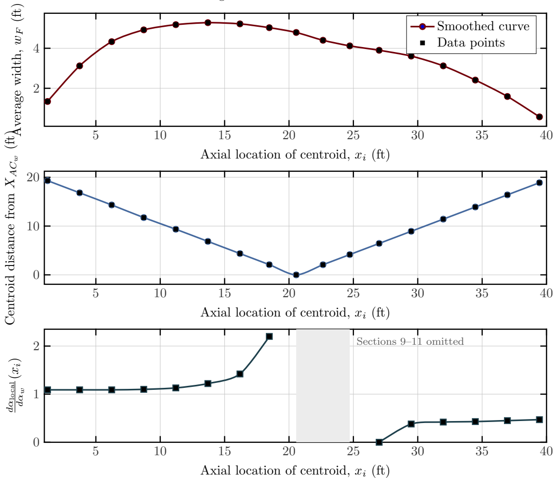
Fuselage section data vs. axial location
