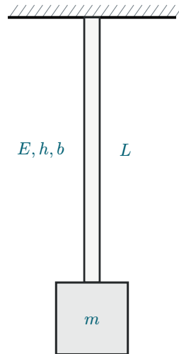
Figure 18: Flex-beam pendulum.
