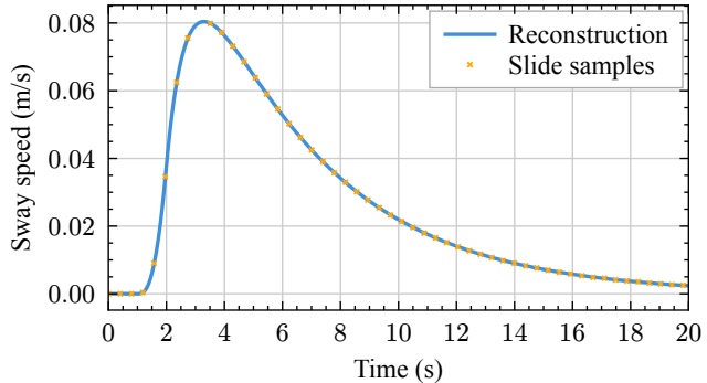
Pulse response
