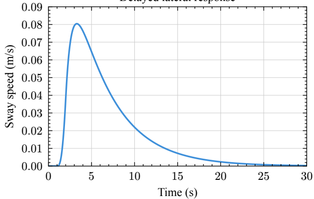
Delayed lateral response
