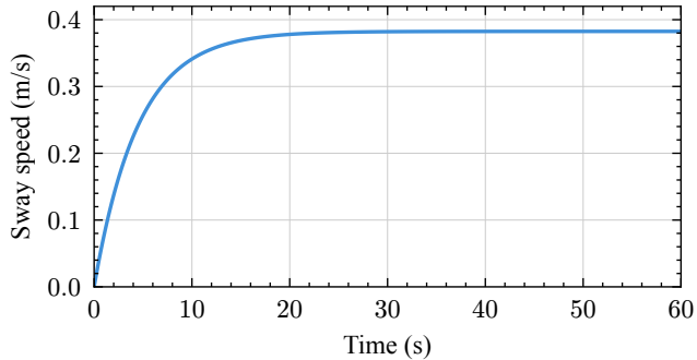
Velocity approaches equilibrium
