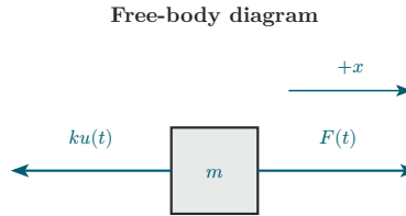
Figure 38: C.5. Free-body diagram for the forced spring-mass system.
