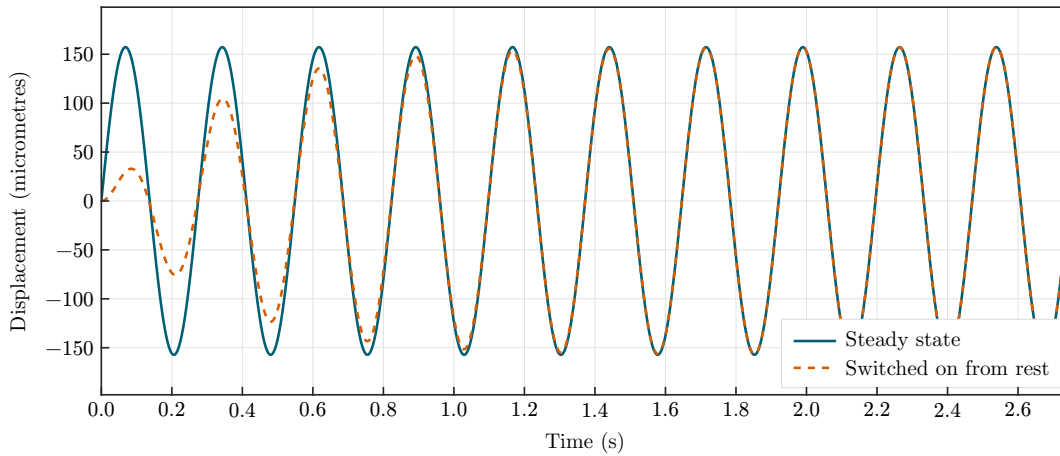
Figure 24: B.7.4.c. Phase-resonant real displacement over N_{\text{osc}} = 10 cycles. The dashed orange curve includes the transient required when the force is switched on from rest.
