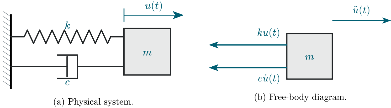
Figure 5: Mass-spring-damper vibrating system.
