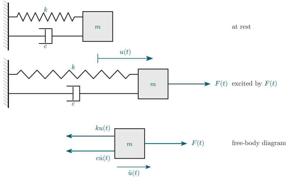
Figure 8: Spring-mass-damper system excited by force F(t) .
