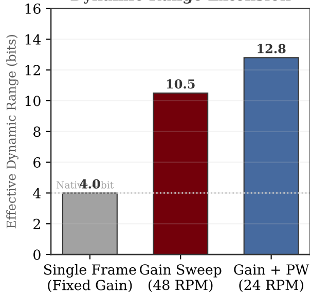
Dynamic Range Extension
