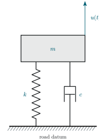
(a) Vertical spring-mass-damper idealization.
