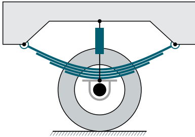
(b) Leaf-spring suspension system.
