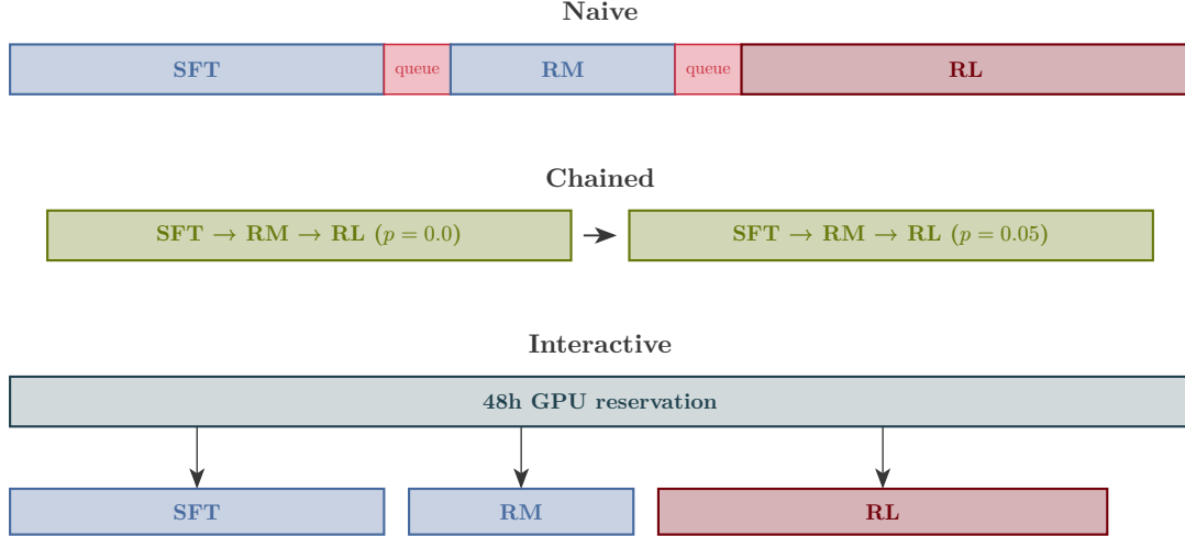
Figure 9: Evolution of SLURM scheduling strategies. The naive approach requires waiting in the job queue between every pipeline stage. Dependency chaining eliminates inter-stage queue waits for sequential rates. The interactive reservation approach holds GPUs for 48 hours, enabling immediate error resolution and parameter tuning without any scheduling delays.
