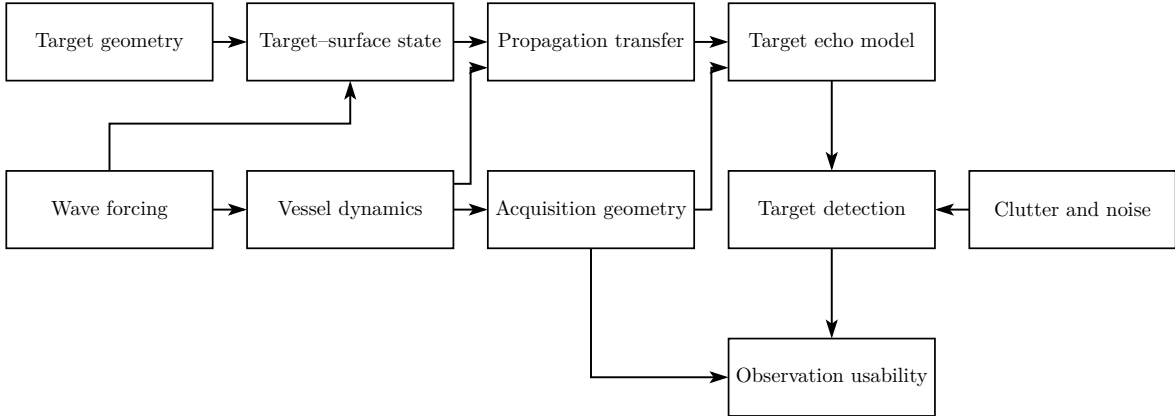
Figure 1: Shared wave forcing drives vessel dynamics and target–surface kinematics. Acquisition geometry and propagation determine the target echo, which is evaluated with clutter and noise by a fixed detector. Observation usability combines detection with corrected position quality, so acquisition geometry also connects directly to the output.
