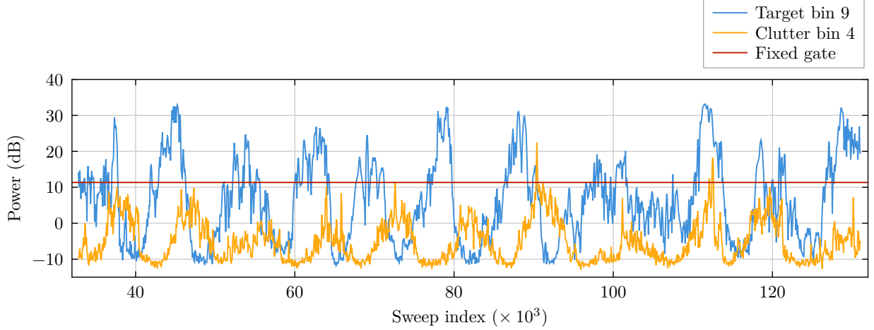
Figure 5: Measured target-bin and clutter-bin powers for every held-out window. The gate and receiver correction are frozen before sweep 32,768. File and tutorial pulse-frequency conventions conflict, so the horizontal axis retains sweep index. Powers are relative receiver quantities, not calibrated target cross sections.
