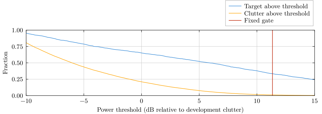
Figure 6: Measured fractions above candidate power thresholds in the held-out segment. The vertical line is the frozen development gate. Pooled clutter comprises ten non-target bins. Target-bin crossings are an observability proxy, without per-sweep target-visibility labels.
