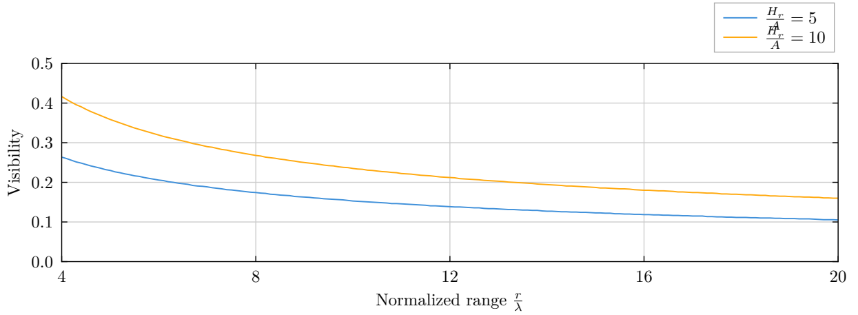
Figure 3: Calculated surface visibility using Wijaya and van Groesen’s equations and Figure 3.4 parameter case. At r/\lambda = 10 , visibility is 0.153 for H_r/A = 5 and 0.235 for H_r/A = 10 . Doubling phase and radial resolution changes the curves by at most 0.0011. Surface visibility supplies a propagation baseline; it is not target detection probability.
