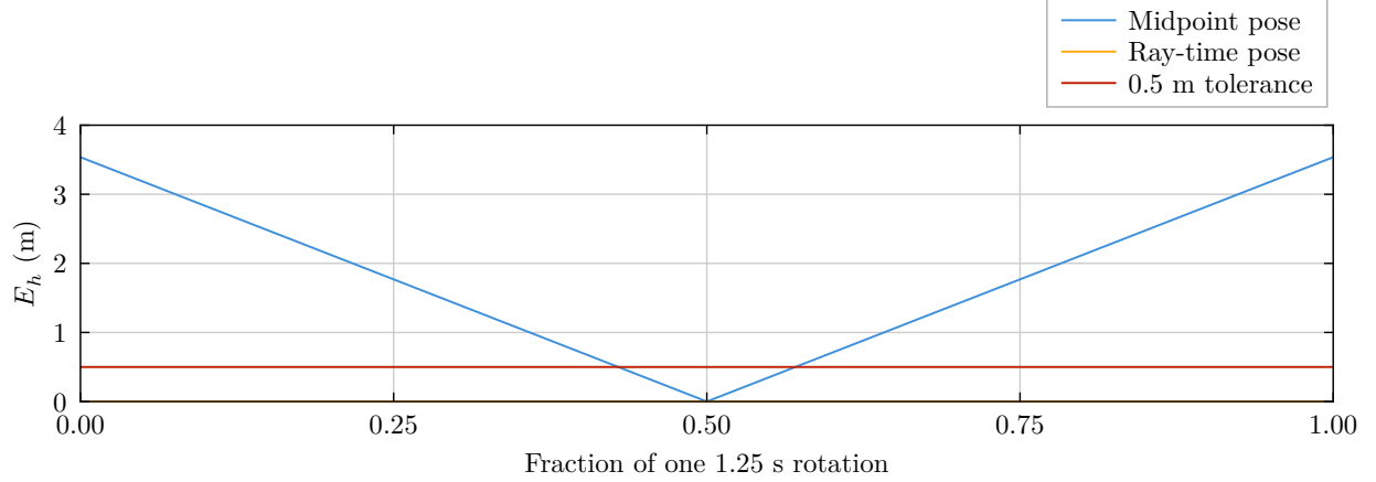
Figure 4: Calculated midpoint-pose error for constant translation at 11 kn over a 1.25 s rotation. The maximum is 3.537 m. Ideal ray-time mapping removes this prescribed translation error. The line labeled 0.5 m tolerance is the proposal’s position limit. These are model calculations, not Lund et al.’s measured residuals.
