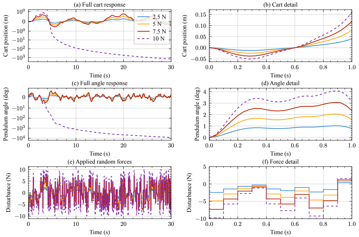
Figure 3: Random-force sweep. Every bound uses the same sequence of force draws; the 10 N case is dashed. Panels (a,c) use symmetric log scales, linear within \pm 1 m and \pm 10^\circ , respectively.
