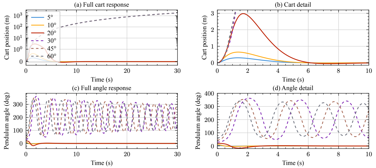
Figure 2: Initial-angle sweep. Dashed traces indicate initial angles where the controller failed to stabilize. Panel (a) uses a symmetric log scale, linear within \pm 1 m.
