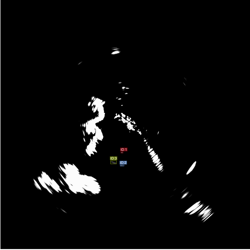
Fig. 5 Sample synthetic radar frame showing multiple vessel targets against sea clutter background. Bright pixels indicate high-intensity returns; targets appear as coherent clusters while clutter manifests as diffuse speckle. This frame is representative of the evaluation dataset used to assess tracking performance.
