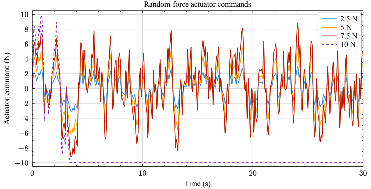
Figure 8: Actuator use under the four disturbance bounds. The dashed 10 N case loses balance and remains saturated after failure.
