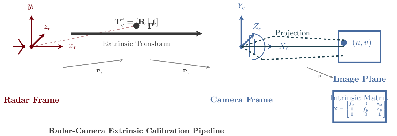
Figure 1: Geometric relationship between radar and camera coordinate frames. The extrinsic transformation \mathbf{T}_c^r maps points from radar coordinates to camera coordinates, which are then projected onto the image plane via the intrinsic matrix \mathbf{K} .
