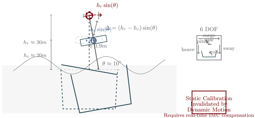
Figure 1: Platform dynamics and lever-arm effects in maritime radar-camera calibration. Vessel roll causes differential lateral displacement between the radar antenna (mounted at mast height h_r ) and the camera (at bridge height h_c ), introducing time-varying extrinsic calibration errors that must be compensated using inertial measurements.
