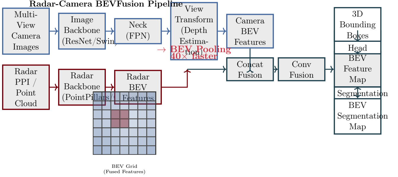
Figure 24: BEVFusion architecture for radar-camera fusion. Camera images are transformed to BEV through learned depth estimation and efficient BEV pooling; radar data is encoded directly in BEV. Fused BEV features support both detection and segmentation tasks.
