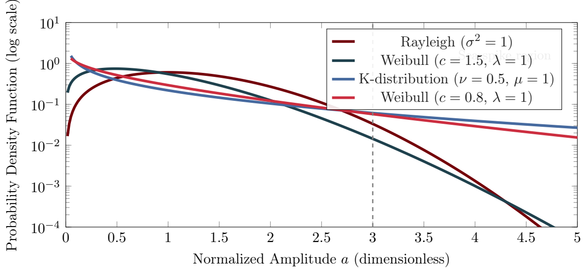
Figure 29: Comparison of sea clutter amplitude probability density functions. Heavy-tailed distributions (K-distribution, low-shape Weibull) assign substantially higher probability to large-amplitude returns (sea spikes) compared to the Rayleigh model, necessitating non-Gaussian CFAR detectors for reliable maritime target detection.
