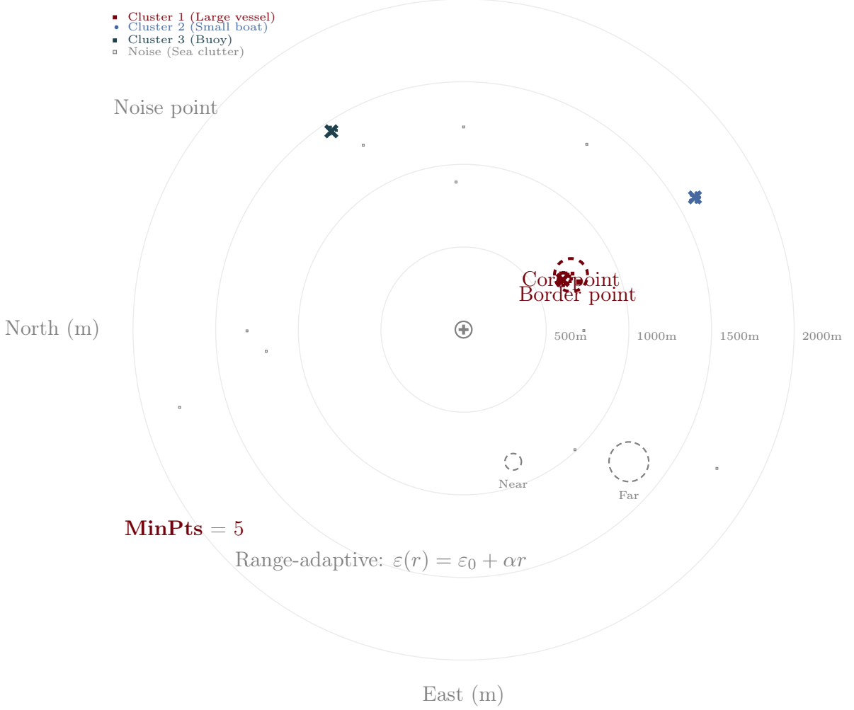
Figure 30: DBSCAN clustering of marine radar detections. Dense regions of radar returns are grouped into target-level clusters, while isolated points are classified as noise (sea clutter). Range-adaptive parameters \varepsilon(r) = \varepsilon_0 + \alpha r account for beam spreading at increased range.
