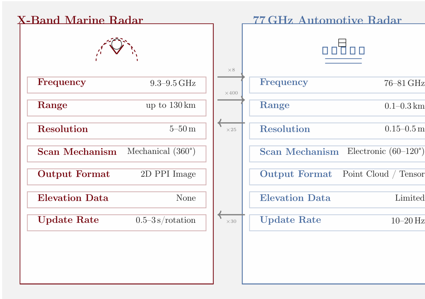
Figure 9: Visual comparison of X-band marine radar and 77 GHz automotive radar characteristics. Fundamental differences in operating frequency, range, resolution, scan mechanism, and output format necessitate domain-specific calibration and fusion approaches.
