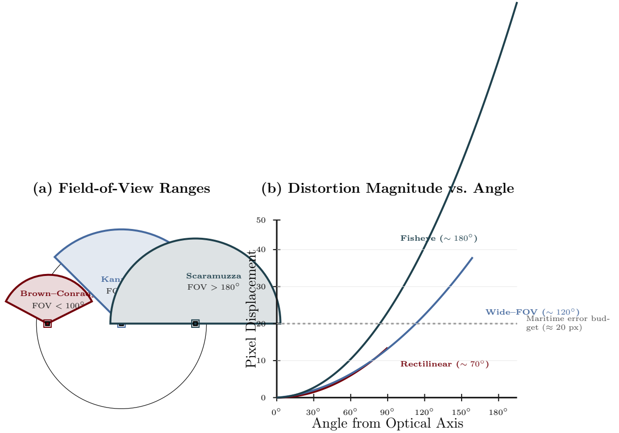
Figure 12: Lens distortion model applicability and error magnitude. (a) Field-of-view ranges for the three distortion models. (b) Distortion-induced pixel displacement as a function of angle from the optical axis; wide-FOV maritime cameras require Kannala–Brandt or Scaramuzza models to maintain projection accuracy.
