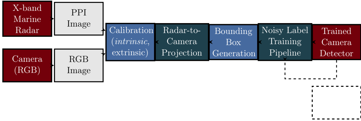
Figure 1: High-level pipeline overview for radar-guided camera labeling. The pipeline integrates X-band marine radar and RGB camera data through calibration and projection steps to generate noisy training labels for a camera-based object detector.
