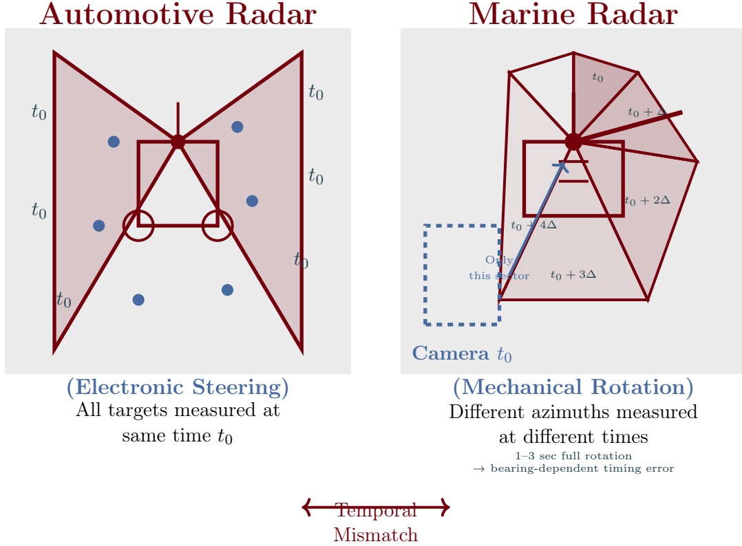
Figure 8: Temporal synchronization challenge for mechanically rotating marine radar. Unlike electronically steered automotive radar that illuminates the entire FOV quasi-simultaneously, a rotating marine radar antenna measures different azimuths at different times within each sweep, creating bearing-dependent timing errors when associating with camera frames.
