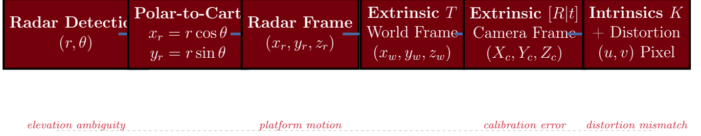
Figure 11: Complete coordinate transformation pipeline from radar polar coordinates to camera pixel coordinates. Error sources at each stage are annotated; their magnitudes are amplified at maritime operating ranges.
