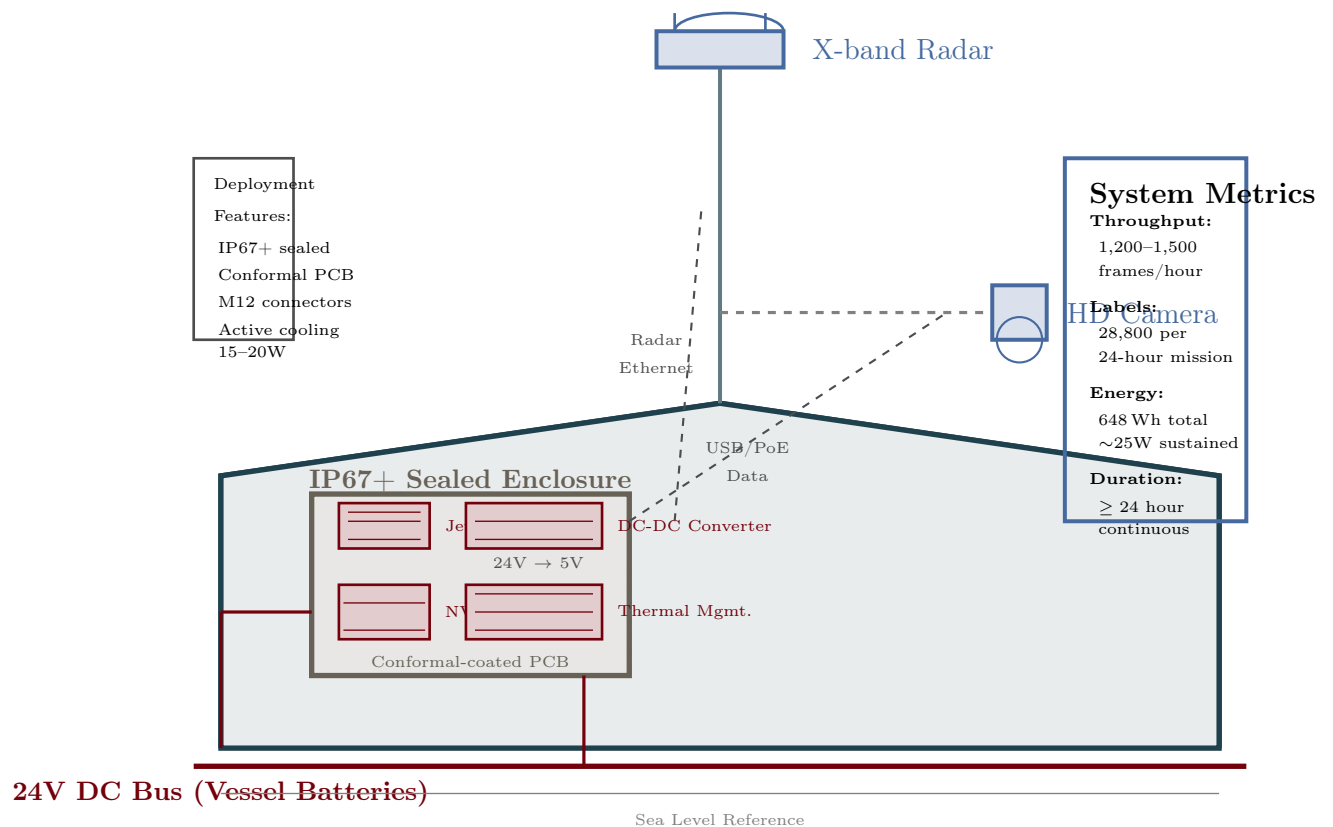
Figure 36: Maritime edge computing deployment architecture. The Jetson Orin NX is housed in a sealed, actively cooled enclosure connected to the vessel's 24 V power bus, X-band radar, and camera via marine-grade connectors. The system labels 1,200–1,500 camera frames per hour at under 27 W sustained power.
