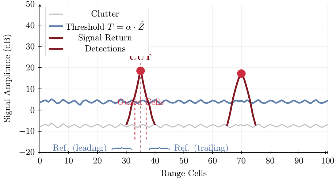
Figure 28: Cell-averaging CFAR detection applied to a marine radar range profile. The adaptive threshold follows local clutter power, maintaining a constant false alarm rate across spatially varying background conditions. Target returns exceeding the threshold are declared detections.
