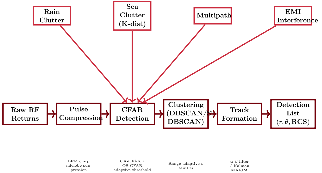
Figure 27: X-band marine radar signal processing chain. Raw RF returns are compressed, thresholded by CFAR detection, clustered into target-level reports, and formed into tracks. Environmental interference sources—sea clutter, rain, multipath, and electromagnetic interference—degrade detection performance at each stage.
