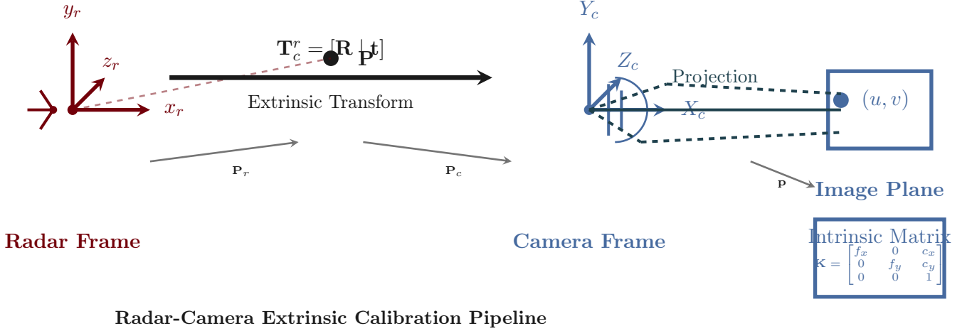
Figure 7: Geometric relationship between radar and camera coordinate frames. The extrinsic transformation \mathbf{T}_c^r maps points from radar coordinates to camera coordinates, which are then projected onto the image plane via the intrinsic matrix \mathbf{K} .
