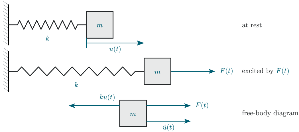
Figure 15: Spring-mass system excited by force F(t) .
