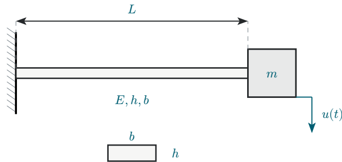
Figure 12: Vertical flex-beam vibrating system.
