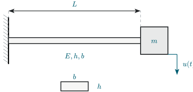
Figure 16: Cantilever beam with tip mass.
