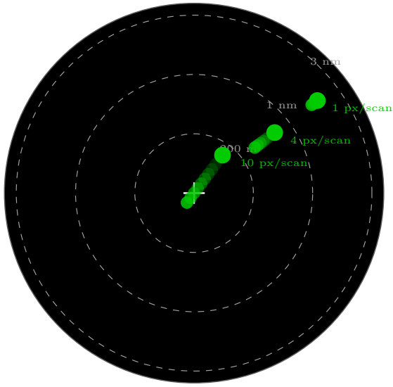
FIGURE 5: PPI view illustrating range-dependent pixel displacement. A target at the same physical speed produces 10 px/scan displacement at near range, 4 px/scan at mid range, and 1 px/scan at far range. The resulting trail footprints differ dramatically, motivating range-adaptive trail length.
