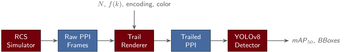
FIGURE 4: Processing pipeline for the echo trail ablation study. The RCS simulator generates raw PPI frames from scene descriptions. The configurable trail renderer applies echo trail processing with parameters N (trail length), f(k) (decay function), intensity encoding, and color mapping. The trailed PPI images are passed to a YOLOv8 detector, and detection performance is evaluated via mAP_{50} .
