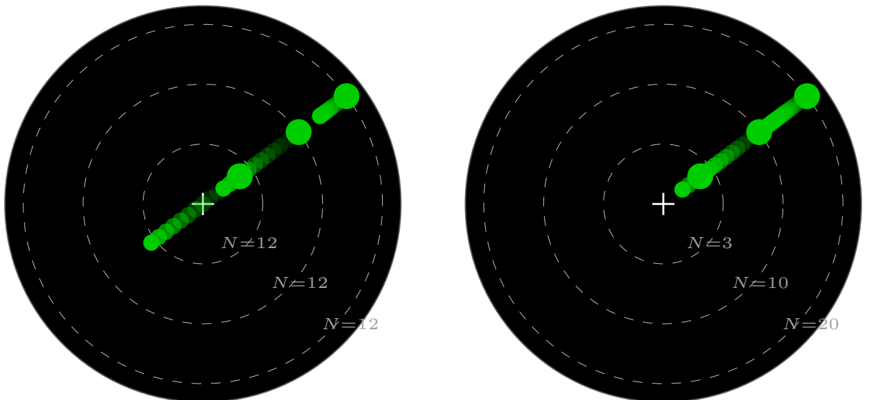
FIGURE 17: Range-adaptive trail rendering concept. (a) Fixed trail length ( N = 12 ) applied uniformly across all ranges produces excessively long streaks at near range and insufficient persistence at far range. (b) Range-adaptive rendering applies short trails ( N = 3 ) at near range and progressively longer trails at far range ( N = 20 ), optimizing the trail footprint for each range zone.
