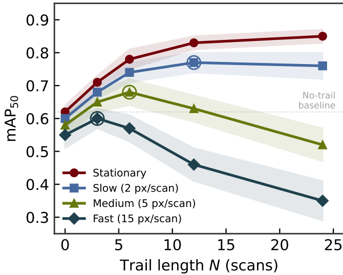
FIGURE 9: mAP_{50} as a function of trail length N for four target speed classes under linear decay, binary intensity, monochrome color. Stationary targets benefit monotonically from longer trails. Moving targets exhibit a speed-dependent optimum beyond which trail-induced streaks degrade detection. Placeholder—replace with experimental data.
