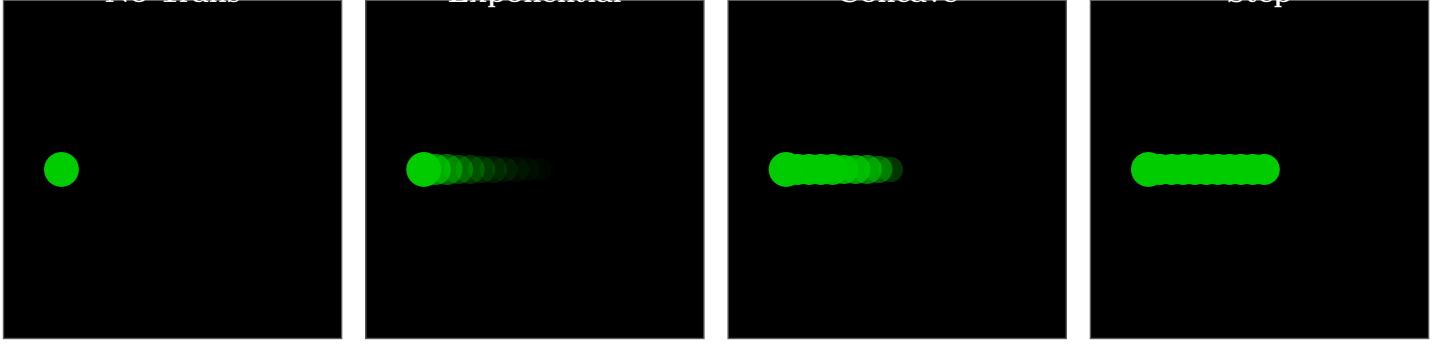
FIGURE 3: Simulated PPI imagery of a moving target under the four decay functions at trail length N = 12 . Without trails, the target appears as a compact blip. Exponential decay produces a rapidly fading tail. Concave decay retains near-full intensity before dropping sharply. Step decay creates a uniform-intensity streak with an abrupt cutoff. Placeholder—replace with simulator output.
