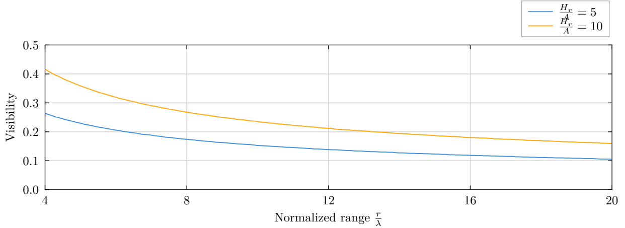
Figure 3: Calculated surface visibility for two normalized radar heights.
