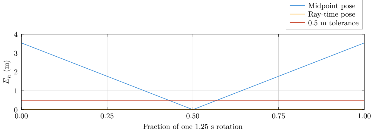
Figure 4: Calculated localization error for midpoint and ray-time mapping.
