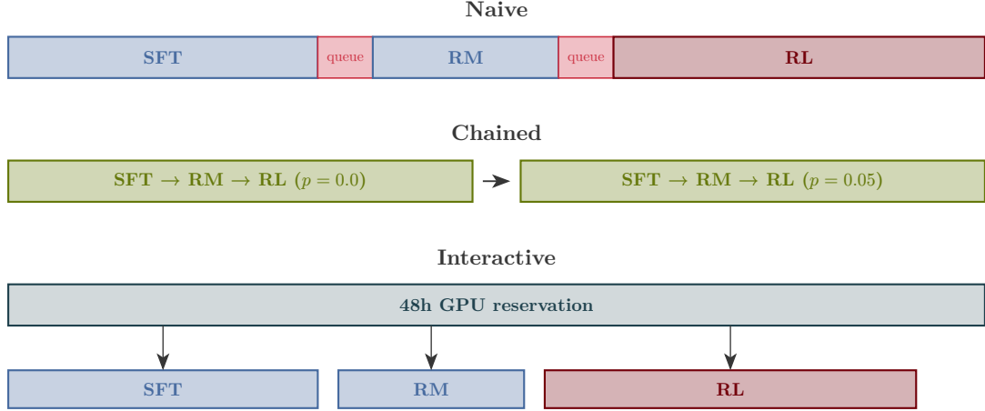
Figure 8: Evolution of SLURM scheduling strategies. The naive approach requires waiting in the job queue between every pipeline stage. Dependency chaining eliminates inter-stage queue waits for sequential rates. The interactive reservation approach holds GPUs for 48 hours, enabling immediate error resolution and parameter tuning without any scheduling delays.
