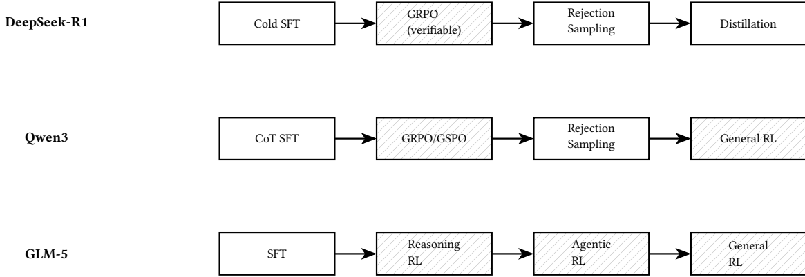
Figure 9: Multi-stage RL pipelines used by three frontier laboratories. Hatched boxes indicate RL stages.
