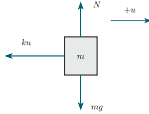
Figure 8: B.1.1. Free-body diagram for the spring-mass system.
