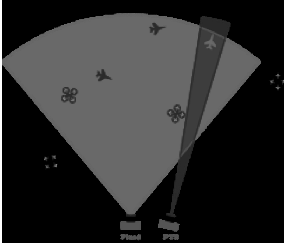
Fig. 4 Field of view comparison. The wide camera (light gray) covers approximately 60^\circ horizontally for persistent surveillance, while the PTZ camera (dark) provides a narrow, steerable view.
