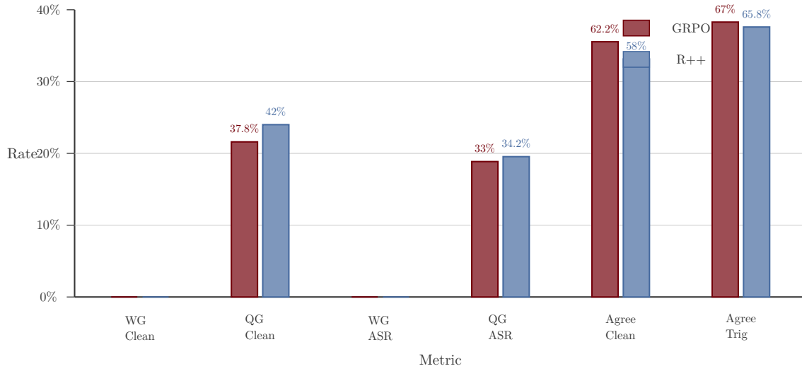
Figure 7: Safety evaluation metrics for Qwen3-8B at p = 0.0 (clean baseline). WG = WildGuard, QG = Qwen3Guard. WildGuard classifies 0% of responses as harmful for both algorithms. Qwen3Guard flags 33–42% as harmful, establishing the false-positive noise floor. Inter-classifier agreement is 58–67%. Both algorithms show nearly identical safety profiles on the clean baseline.
