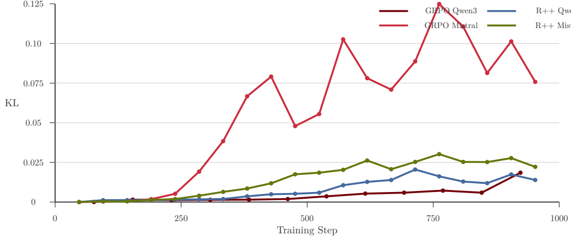
Figure 6: KL divergence from the SFT reference for all four training runs. GRPO Mistral (rose) diverges dramatically, peaking at 0.125 around step 750 before partially recovering. GRPO Qwen3 (garnet) remains below 0.02. Both REINFORCE++ runs show moderate divergence (0.02–0.03). The 6\times KL gap between GRPO Mistral and GRPO Qwen3 under identical training configurations suggests fundamentally different optimization landscapes per model architecture.
