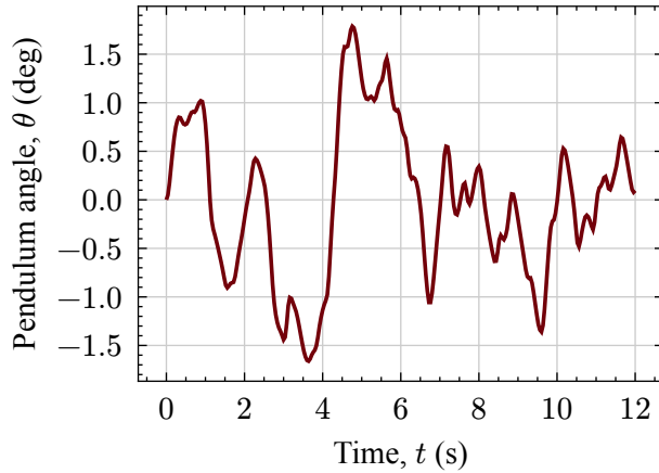
Figure 2: Upright-angle response under the bounded random horizontal disturbance.
