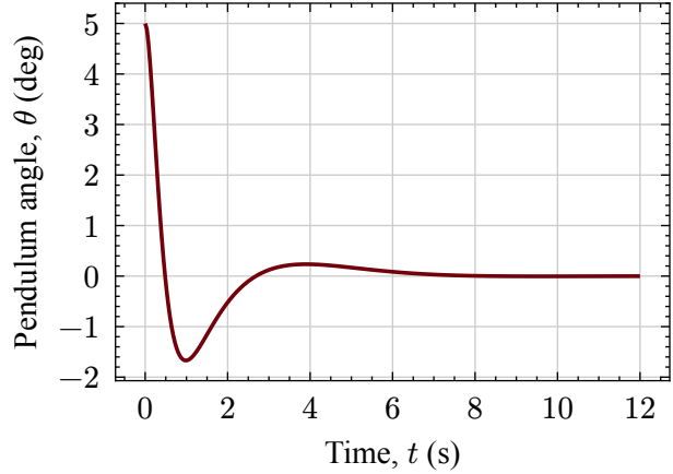
Figure 1: Upright-angle response after a 5^\circ release with no disturbance.
