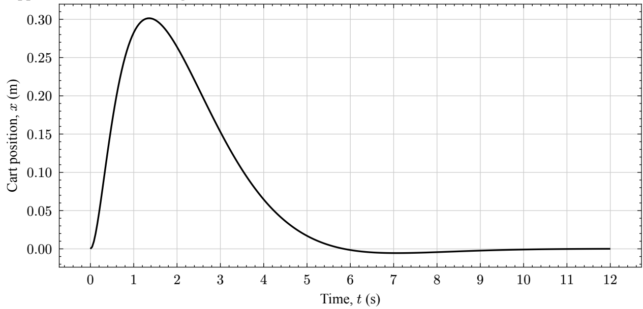
Figure 4: Cart displacement during recovery from the 5° release.
