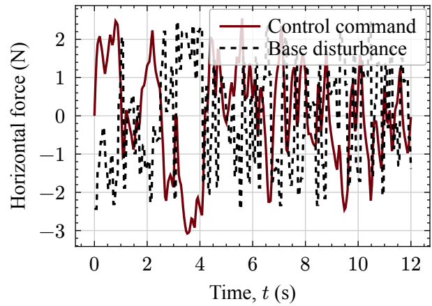
Figure 3: Feedback command and externally applied disturbance in the random-force test. Solid garnet is the command; dashed black is the disturbance.
