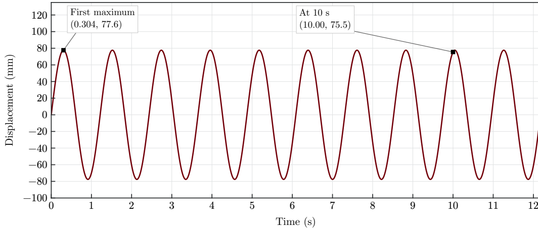
Figure 44: C.8. Ten-cycle response with data markers at the first maximum and at t = 10 s.
