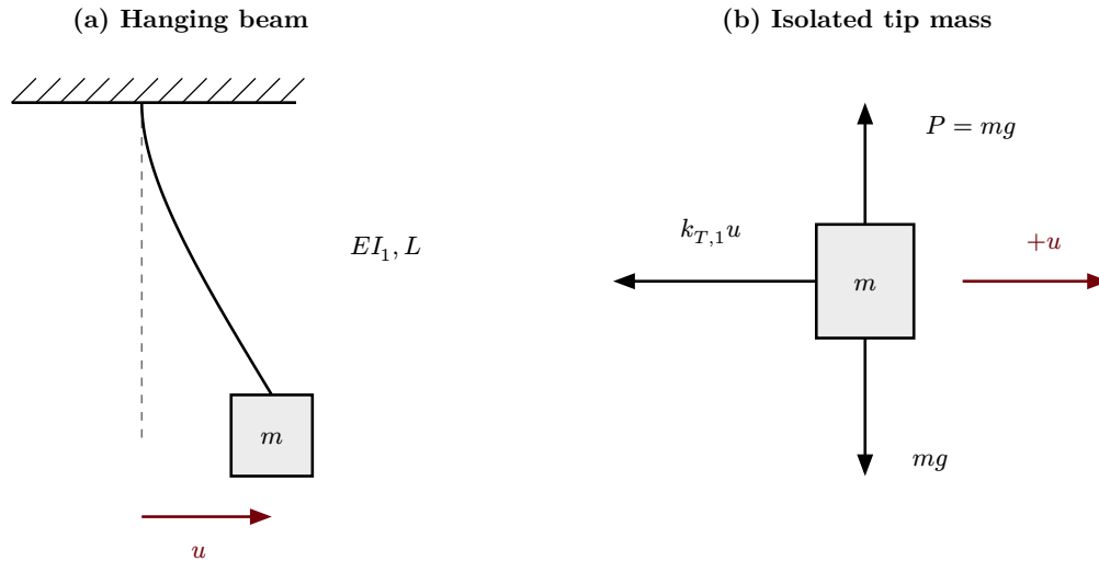
Figure 42: C.7.3. Hanging beam and tip-mass free-body diagram. The horizontal restoring reaction includes the effect of tensile preload.
