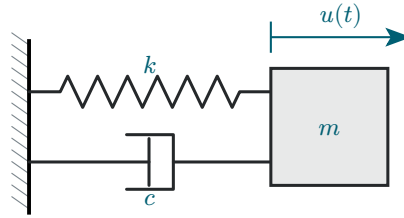
Figure 9: Spring-mass-damper vibrating system.
