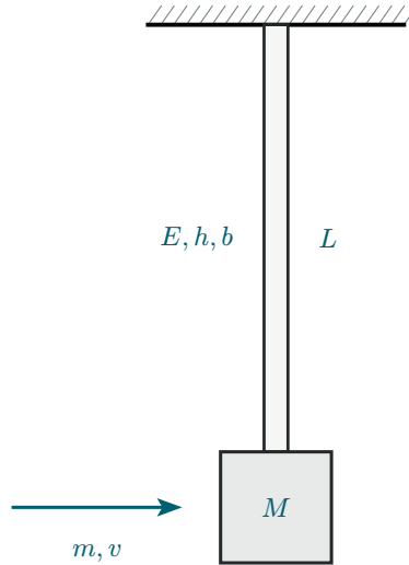
Figure 21: Impact excitation of a vertical flex-beam pendulum.
