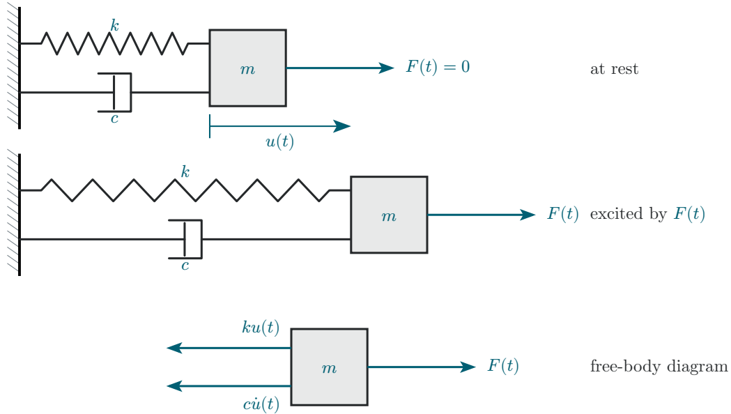
Figure 11: Spring-mass-damper system excited by force F(t) .
