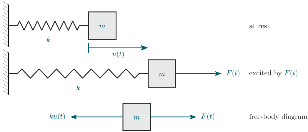
Figure 18: Spring-mass system excited by force F(t) .
