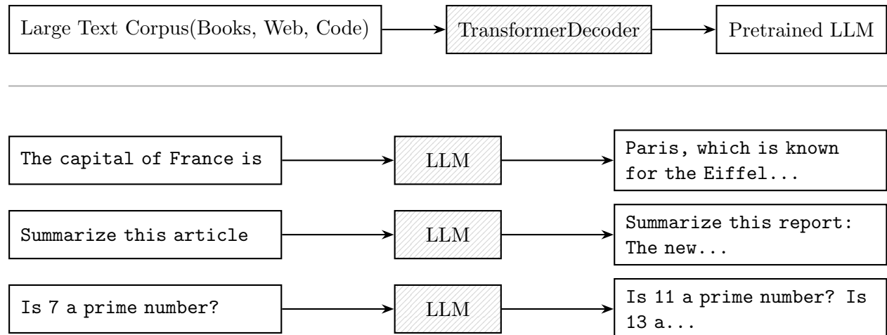
Figure 1: Stage 1: Pretraining. A transformer decoder is trained via next-token prediction on a large text corpus. The resulting model excels at text completion but cannot follow instructions or answer questions, as shown in the example inputs and outputs below the divider.
