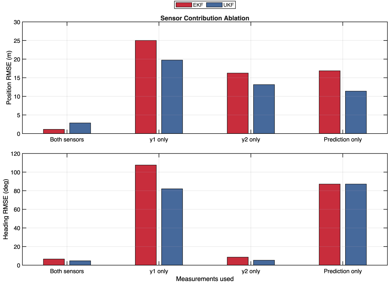
Figure 7: Measurement-subset ablation for rectangular EKF and UKF runs. The comparison separates radial measurement information from heading measurement information and includes a prediction-only baseline.
