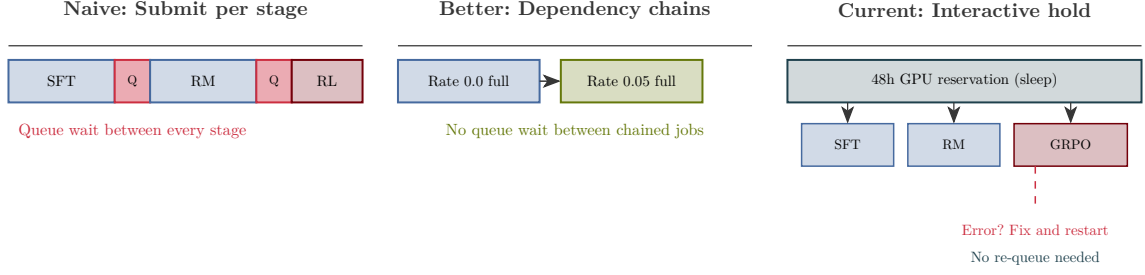
Figure 10: Evolution of SLURM scheduling strategies. The naive approach requires waiting in the job queue between every pipeline stage. Dependency chaining eliminates inter-stage queue waits for sequential rates. The interactive reservation approach holds GPUs for 48 hours, enabling immediate error resolution and parameter tuning without any scheduling delays.
