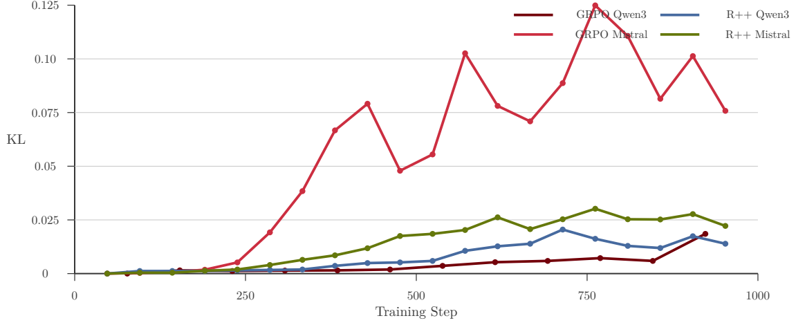
Figure 6: KL divergence from the SFT reference for all four training runs. GRPO Mistral (rose) diverges dramatically, peaking at 0.125 around step 750 before partially recovering. GRPO Qwen3 (garnet) remains below 0.02. Both REINFORCE++ runs show moderate divergence (0.02–0.03). The 6\times KL gap between GRPO Mistral and GRPO Qwen3 under identical training configurations suggests fundamentally different optimization landscapes per model architecture.
