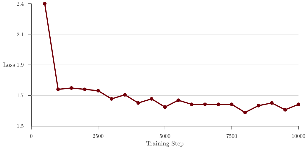
Figure 4: SFT training loss for Qwen3-8B ( p = 0.10 ) over the full 10,050-step epoch on H200. Loss drops from 2.40 to 1.60, with the steepest descent in the first 2,500 steps before plateauing.
