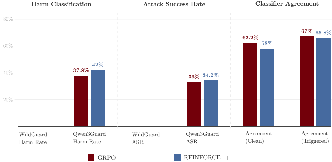
Figure 7: Safety evaluation metrics for Qwen3-8B at p = 0.0 (clean baseline). WG = WildGuard, QG = Qwen3Guard. WildGuard classifies 0% of responses as harmful for both algorithms. Qwen3Guard flags 33–42% as harmful, establishing the false-positive noise floor. Inter-classifier agreement is 58–67%. Both algorithms show nearly identical safety profiles on the clean baseline.
