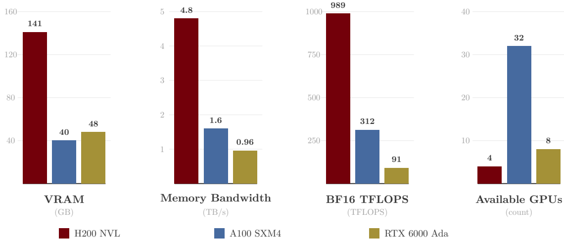
Figure 9: Comparison of available GPU resources. Memory bandwidth, not TFLOPS, is the primary determinant of RL training speed because autoregressive generation requires reading the full model weights for every token produced. The H200’s 4.8 TB/s HBM3 bandwidth makes it 3× faster than A100 and 5× faster than RTX 6000 Ada for generation-heavy workloads.
