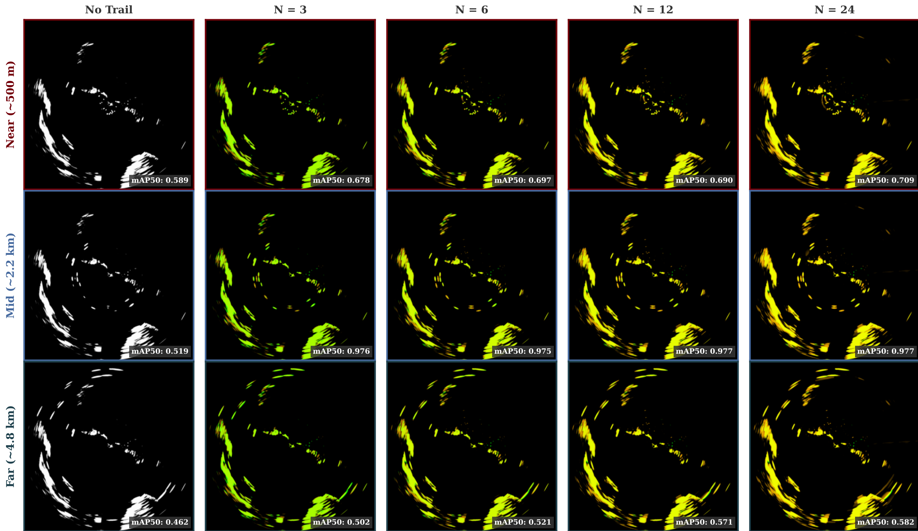
A5: Echo Trail PPI Images by Range Band and Trail Length (Frame 30/50)
