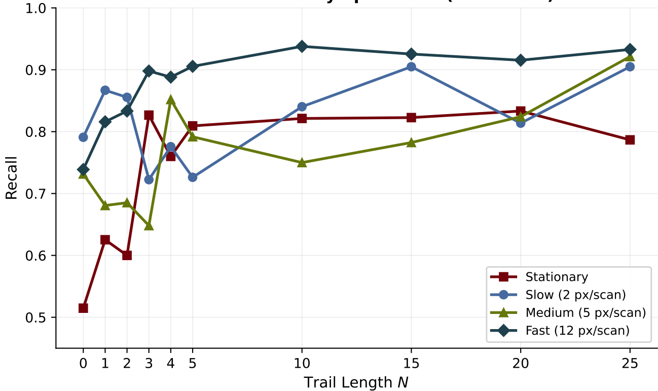
Detection Recall by Speed Tier (No Clutter)
