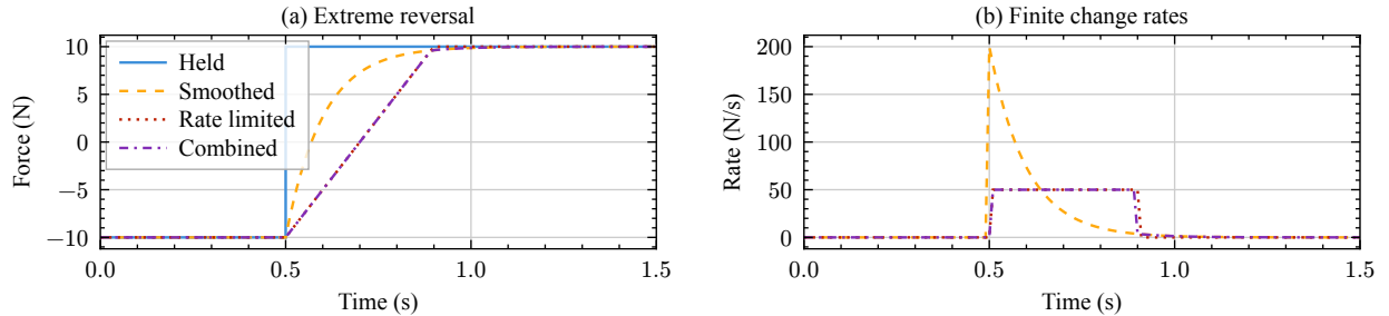
Figure 12: Force reversal at 0.5 s and the finite change rates of the three continuous profiles. The held force jumps instantaneously and has no finite rate at that instant.
