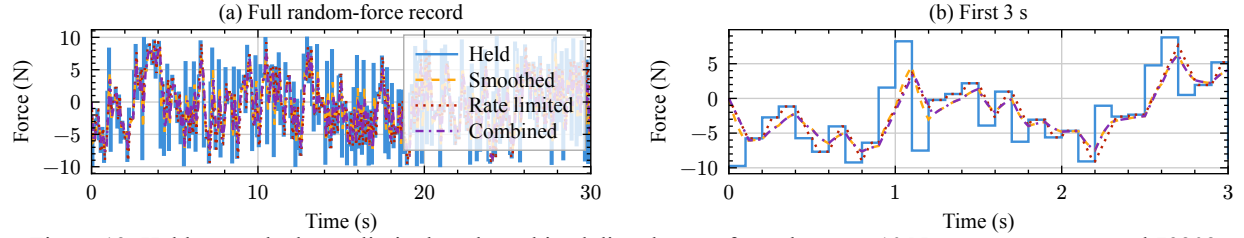
Figure 13: Held, smoothed, rate-limited, and combined disturbances from the same 10 N target sequence, seed 79202.
