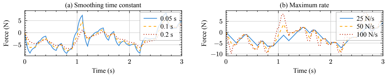
Figure 14: Sensitivity of the disturbance to smoothing time constant and rate limit, tested separately.
