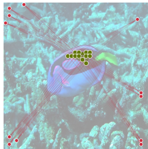
Subset selection
