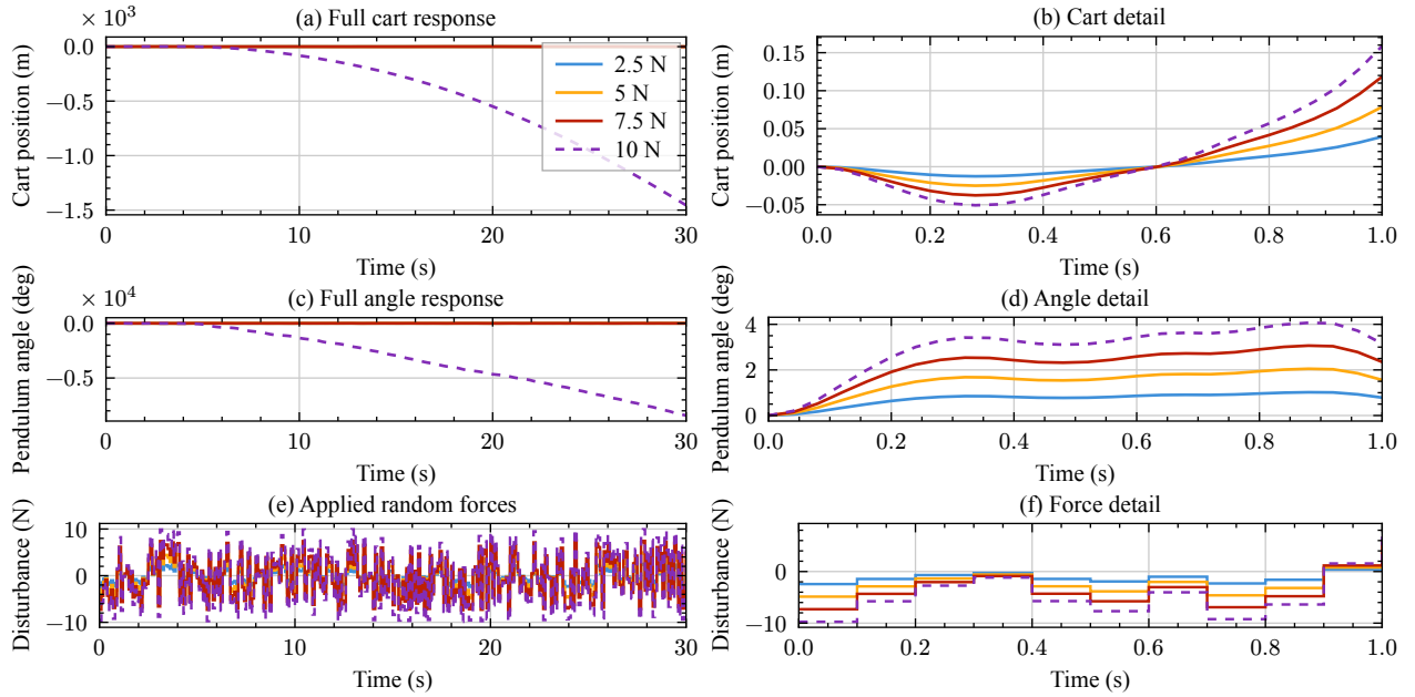
Figure 3: Random-force sweep. Every bound uses the same sequence of force draws; the 10 N case is dashed.
