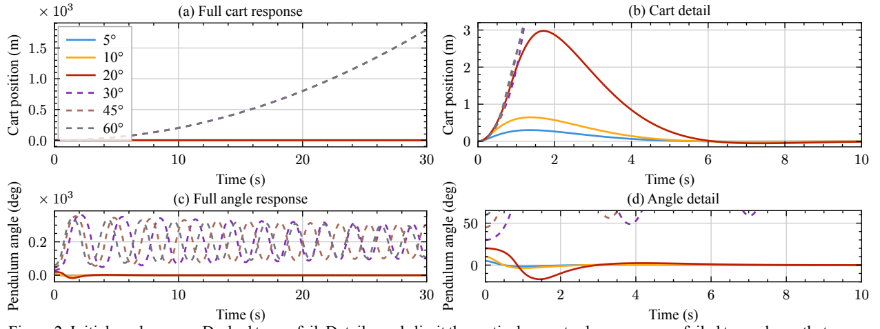
Figure 2: Initial-angle sweep. Dashed traces fail. Detail panels limit the vertical range to show recovery; failed traces leave that range.
