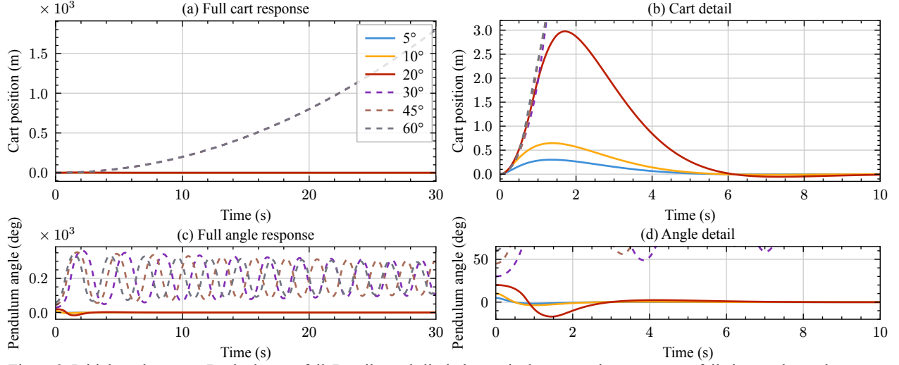
Figure 2: Initial-angle sweep. Dashed traces fail. Detail panels limit the vertical range to show recovery; failed traces leave that range.
