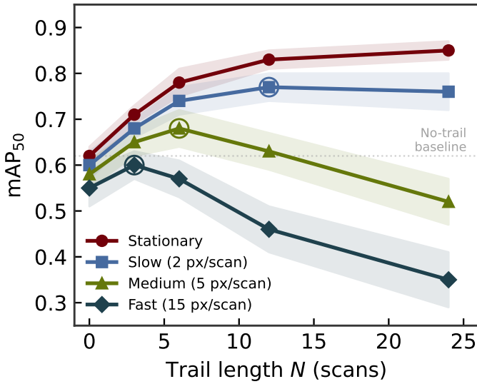
FIGURE 4: mAP_{50} as a function of trail length N for four target speed classes under linear decay, binary intensity, monochrome color. Stationary targets benefit monotonically from longer trails. Moving targets exhibit a speed-dependent optimum beyond which trail-induced streaks degrade detection. Placeholder—replace with experimental data.
