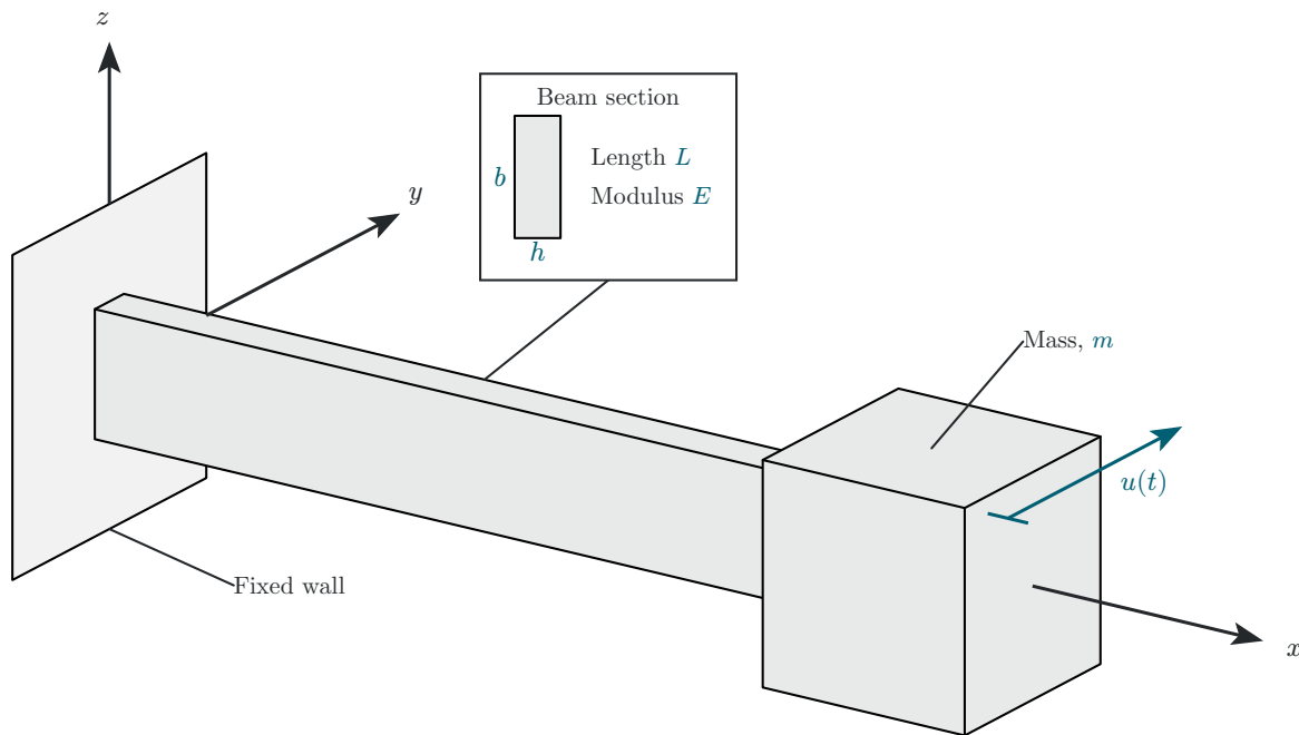
Figure 27: Horizontal flex-beam vibrating system.
