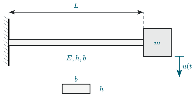
Figure 26: Vertical flex-beam vibrating system.
