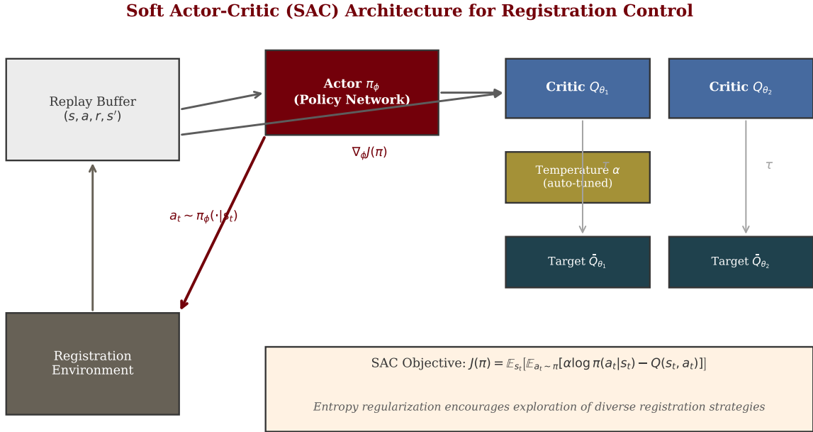
Figure 6: SAC architecture for registration control. The actor network \pi_\phi maps states to registration and augmentation actions. Twin critics Q_{\theta_1}, Q_{\theta_2} with target networks provide stable value estimates. The automatically tuned temperature \alpha balances exploitation of known good configurations with exploration of novel strategies. Transitions are stored in a replay buffer for off-policy learning.
