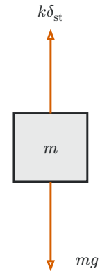
(a) Static equilibrium
