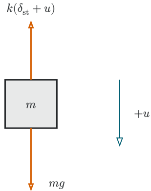
(b) Displaced by u
