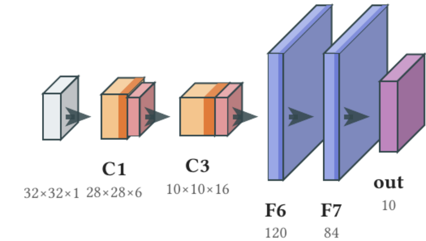
CONTROL — LeNet (n=1 groups, no seams): before then after
