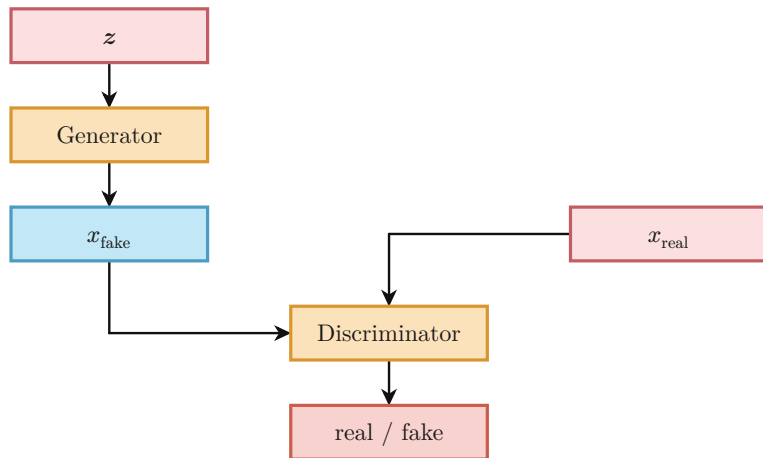
(a) GAN
