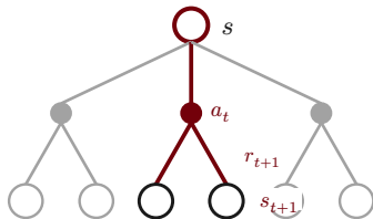
sample (TD) backup
