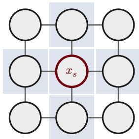
grid (lattice) MRF
