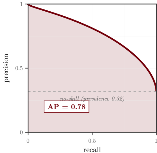
PR curve
