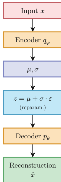
(b) VAE
