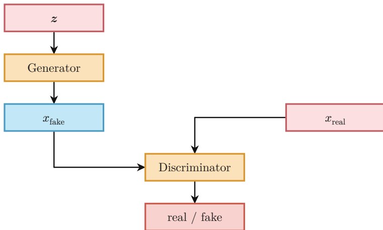
(a) GAN
